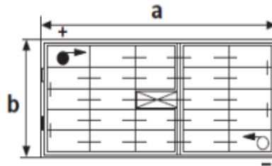
Layout B Circuit B
